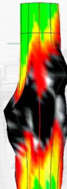
UltraView technology revealed the casing defects (left) in the actual pipe (right) that was pulled from the well
